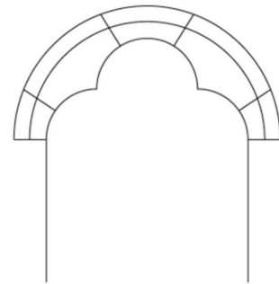
73. Trefoil arch
